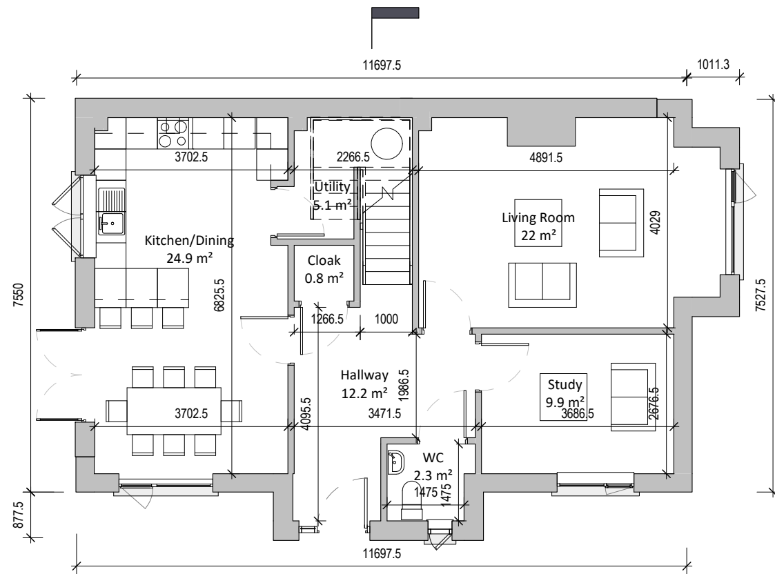
1 H07 Level 00 1 : 100
