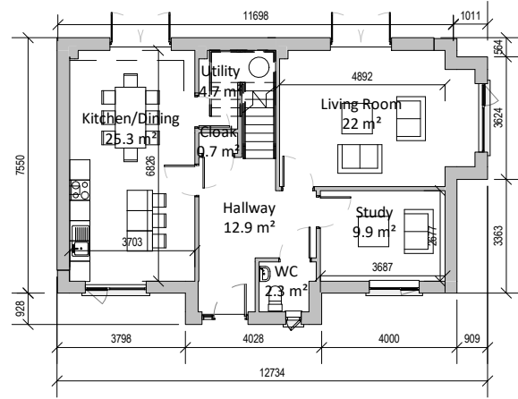
3 H07A Level 00 1 : 200
